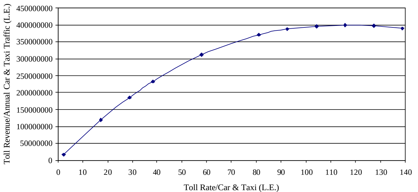
Figure 7: Expected Toll Revenue Versus Varying Toll Rates/Car & Taxi in 2004
